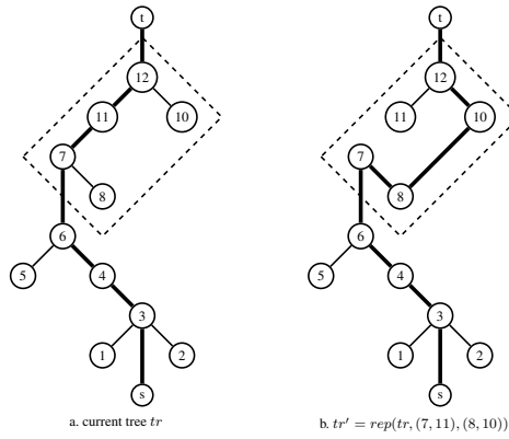
Fig. 2 An Example of Rooted Spanning Tree
