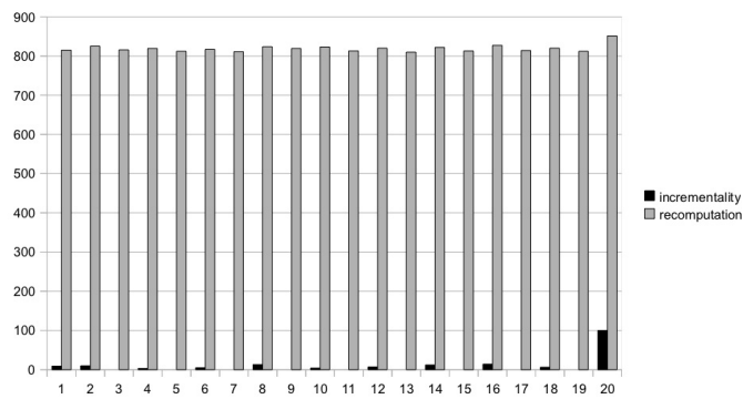
Fig. 6 20 last iterations for a complete graph of size 100
