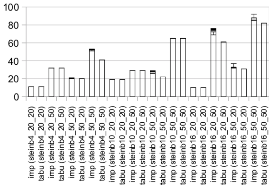
Fig. 18 Comparison between IMP and LS(Graph) on steiner instances
