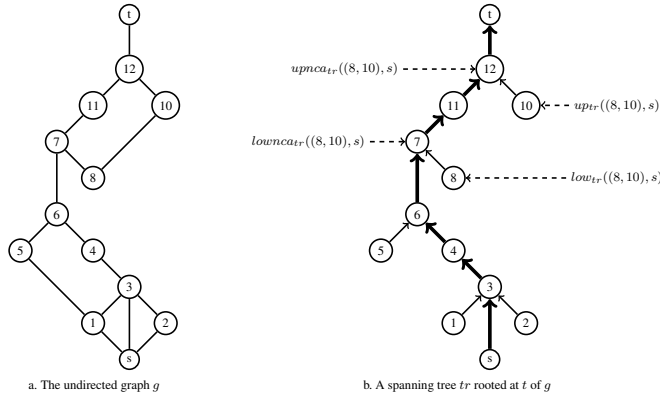
Fig. 2 An Example of Rooted Spanning Tree
