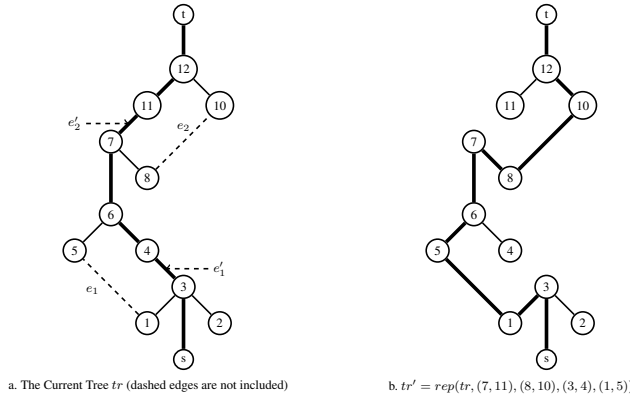
Fig. 4 Illustrating a Complex Move
