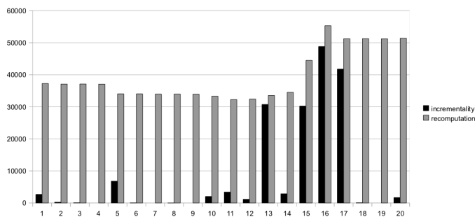
Fig. 7 20 last iterations for a complete graph of size 1000
