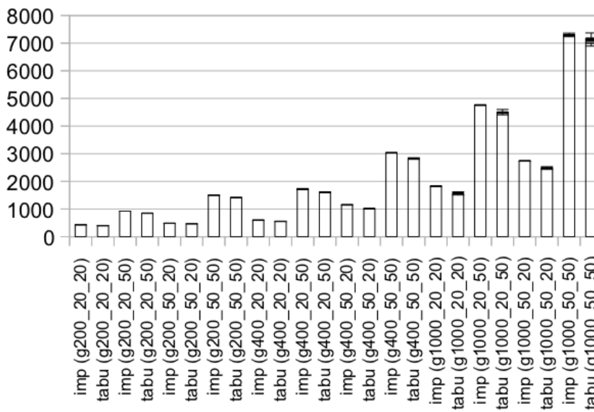
Fig. 17 Comparison between IMP and LS(Graph) on KCT instances
